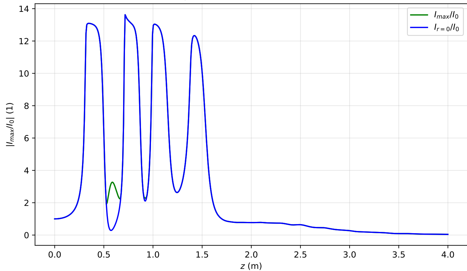
I_{\max}(x = 0, y = 0, z)/I_0 , \text{Pin}=8.5\text{Pcr} , artificial time
